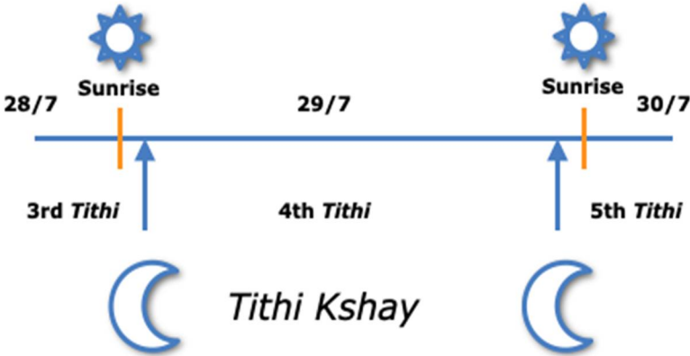
Figure No. 6: tithī kṣaya
