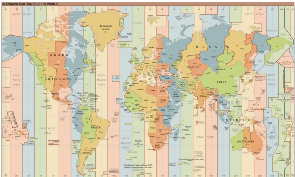
Figure No. 11: Time Zones across the World
