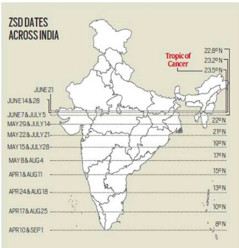
Figure No. 4: Image showing ‘Zero Shadow Day’ taking place in different locations and on different days in India.
