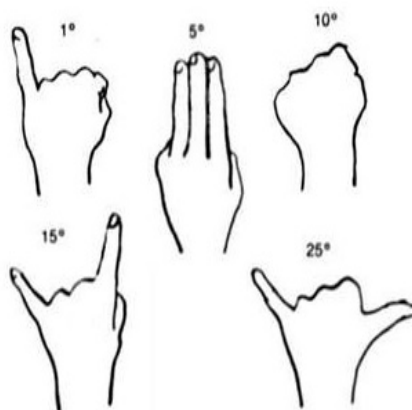
Figure No. 1: Use of fingers to measure celestial angular distance
