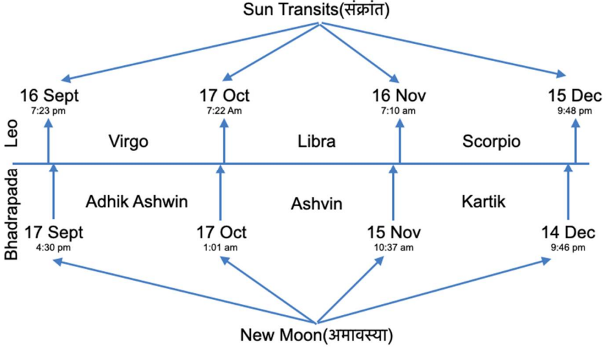
Figure No. 7: Identifying the Adhik Māsa
