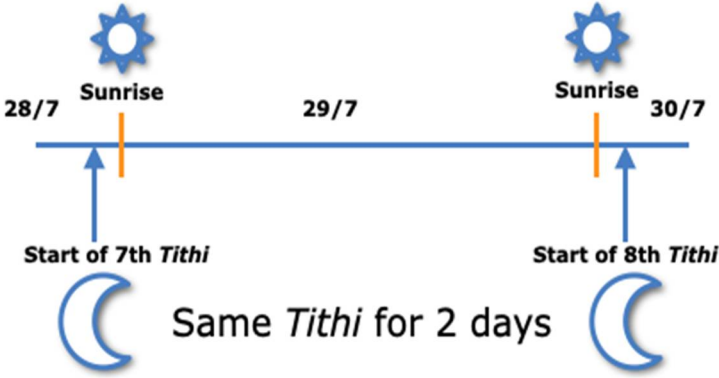
Figure No. 5: tithī vṛddhi
