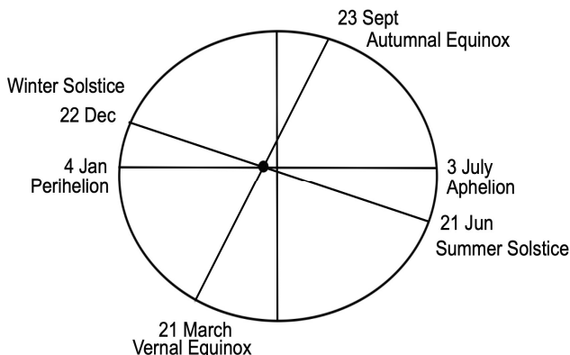
Figure No. 8: The position of the Earth at different days while rotating around the Sun.
