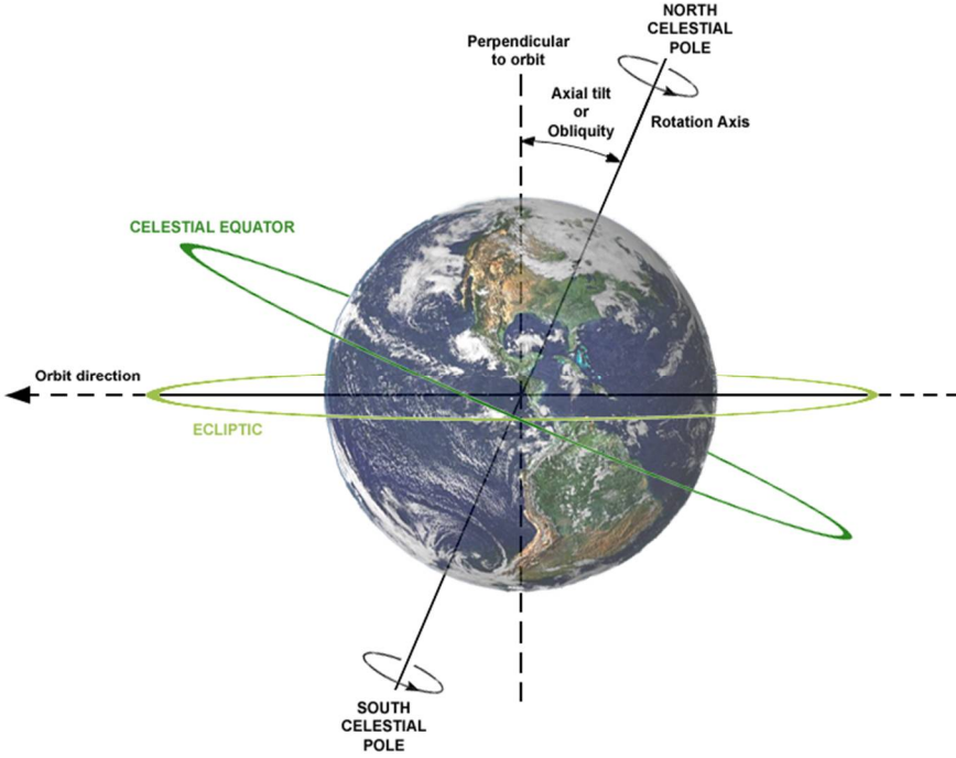
Figure No. 9: Image depicting tilted axis of rotation of the Earth and the tropics.
