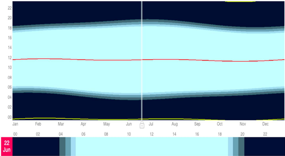
Figure No. 10: Graphical representation of durations of Sunrises and Sunsets over the year.
